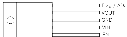
TO220-5L
